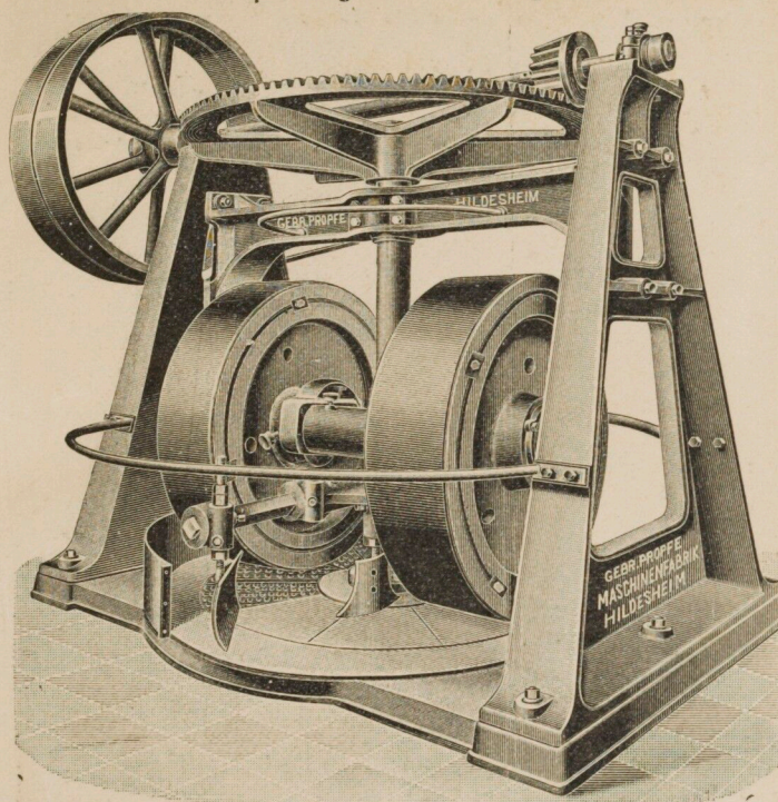
Rollergang.
